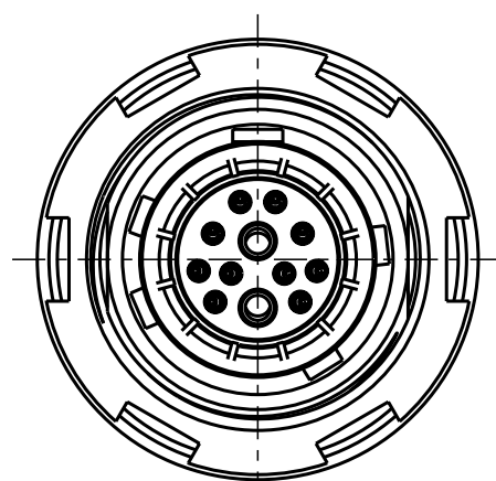
GKOWDM-P12WMMO-000L Mechanical coding: D Color coding: green
