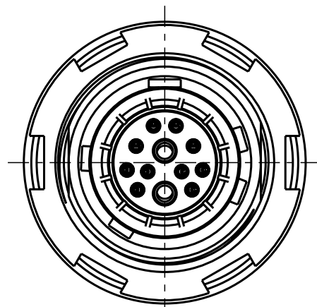
GKOWCM-P12WMMO-000L Mechanical coding: C Color coding: blue
