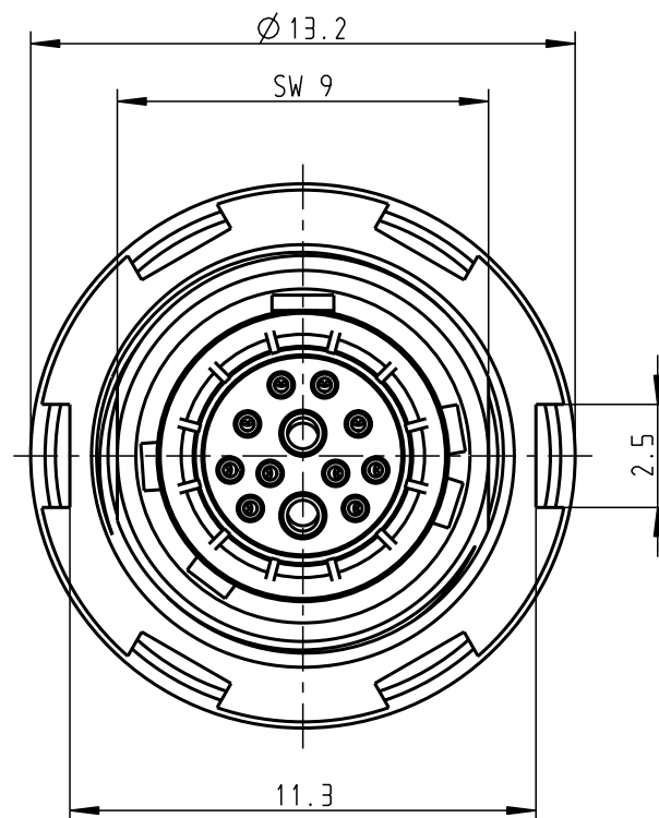
GKOWAM-P12WMMO-000L Mechanical coding: A Color coding: light brown
