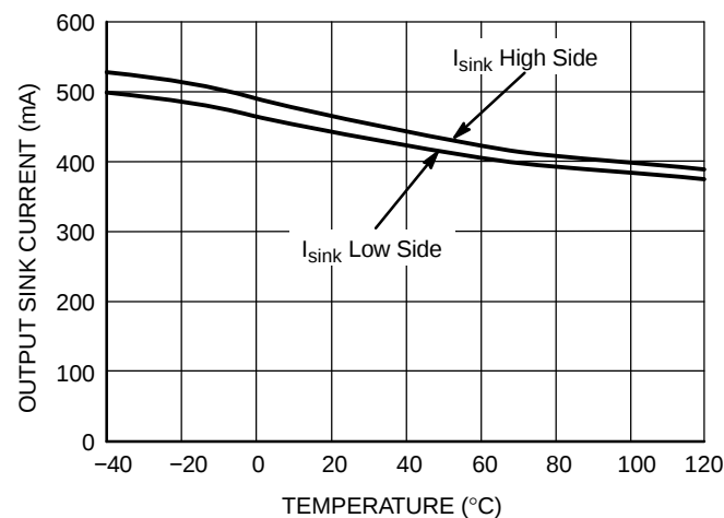
Figure 38. Output Sink Current vs. Temperature
