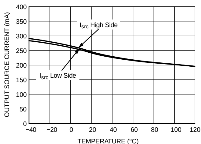
Figure 36. Output Source Current vs. Temperature
