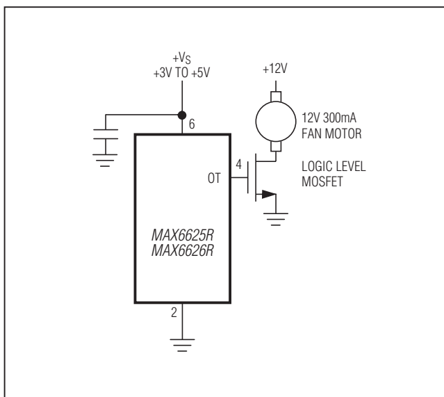
Figure 7. Fan Controller
