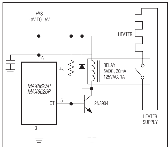
Figure 8. Simple Thermostat
