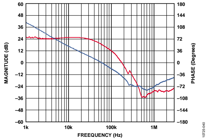
Figure 34. Bode Plot at 4 \text{ A}
