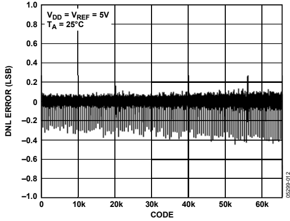
Figure 6. DNL—16-Bit DAC
