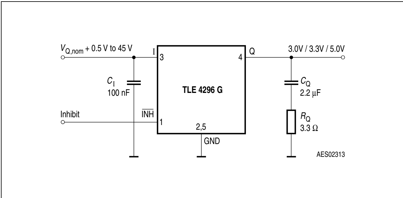
Figure 3 Application Circuit
