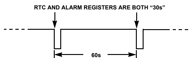
FIGURE 15. \overline{\text{IRQ}}/\text{F}_{\text{OUT}} WAVEFORM
