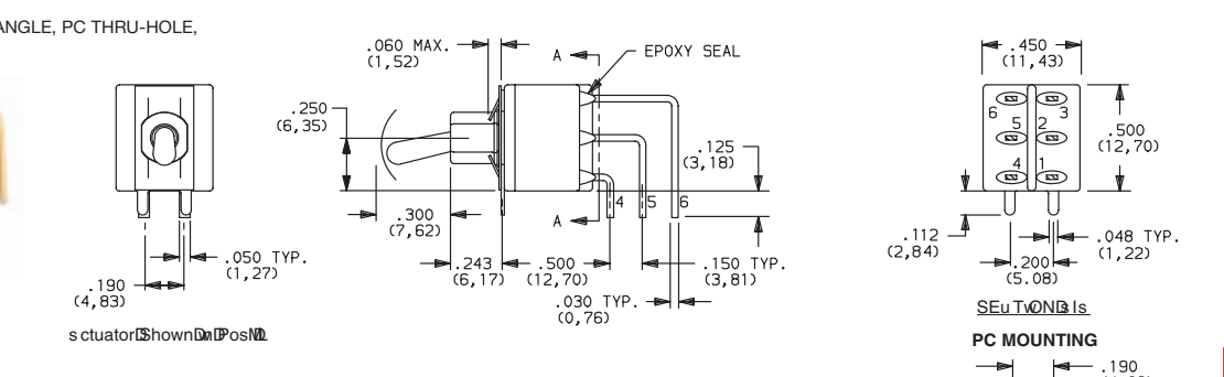
E201MD1AV2BE Vertical Actuation DPDT
