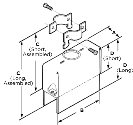
180° Cable Exit
