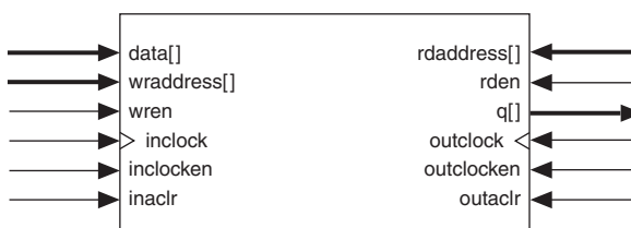
Figure 2–13. Simple Dual-Port & Single-Port Memory Configurations
