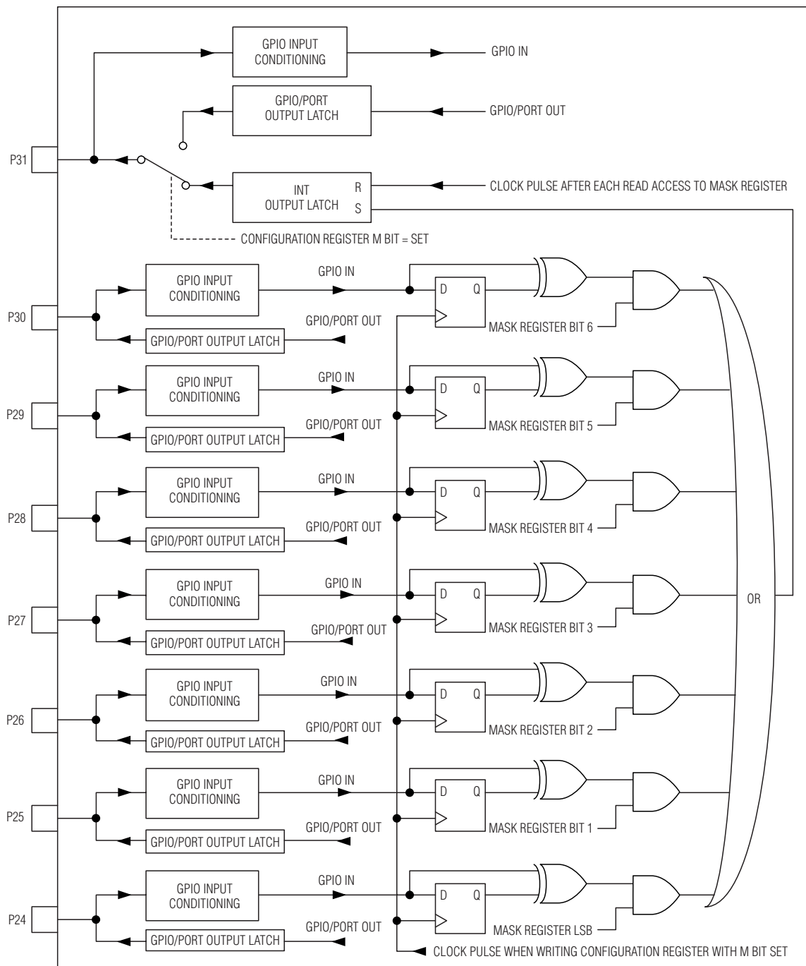
Figure 5. Maskable GPIO Ports P24 Through P31
