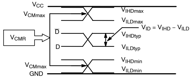
Figure 19. V_{CM} Diagram
