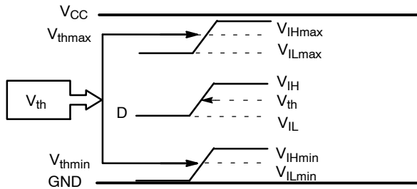
Figure 18. V_{th} Diagram
