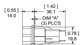
Short Depth - For Solder Termination to PCB
