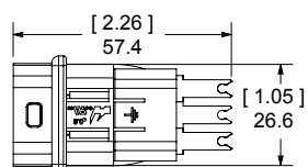
Short Depth - For Solder Termination to Wire
