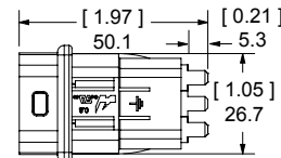
Short Depth - For Solder Termination to PCB
