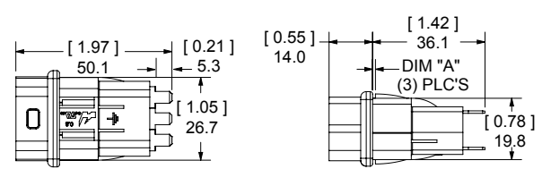
Short Depth - For Solder Termination to PCB
