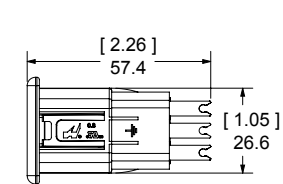
Flush Mount - For Solder Termination to Wire
