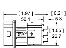
Short Depth - For Solder Termination to PCB
