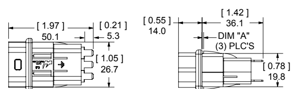
Short Depth - For Solder Termination to PCB
