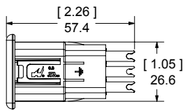
Flush Mount - For Solder Termination to Wire
