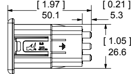
Flush Mount - For Solder Termination to PCB
