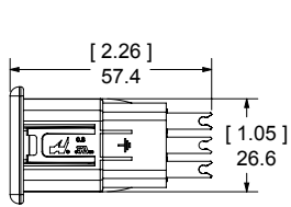
Flush Mount - For Solder Termination to Wire
