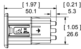
Flush Mount - For Solder Termination to PCB
