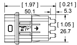
Short Depth - For Solder Termination to PCB
