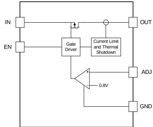
Adjustable Version DFN3030-8 and SOT89-5L
