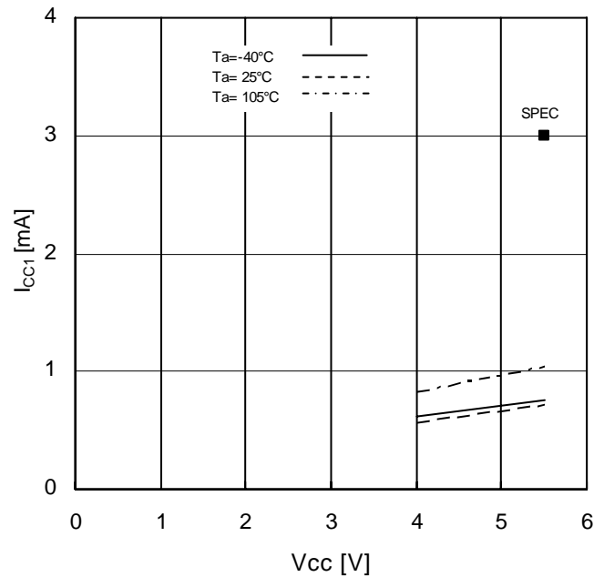
Figure 11. Supply Current (Write) vs Supply Voltage (fSCK=10MHz)
