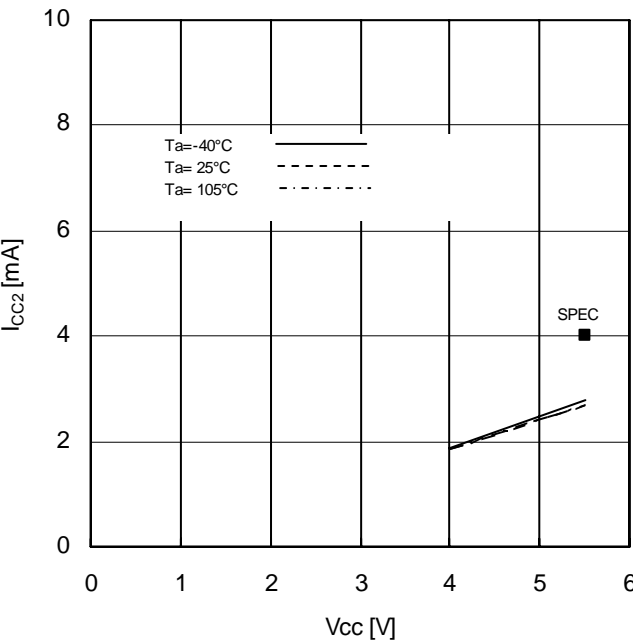
Figure 12. Supply Current (Read) vs Supply Voltage (fSCK=10MHz)
