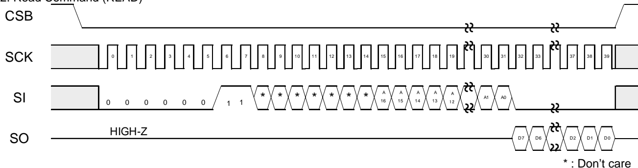
Figure 33. Read command
