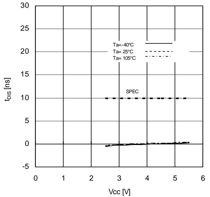
Figure 20. SI Setup Time vs Supply Voltage
