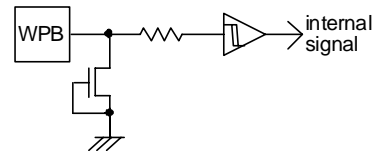
Figure 51. WPB input equivalent circuit
