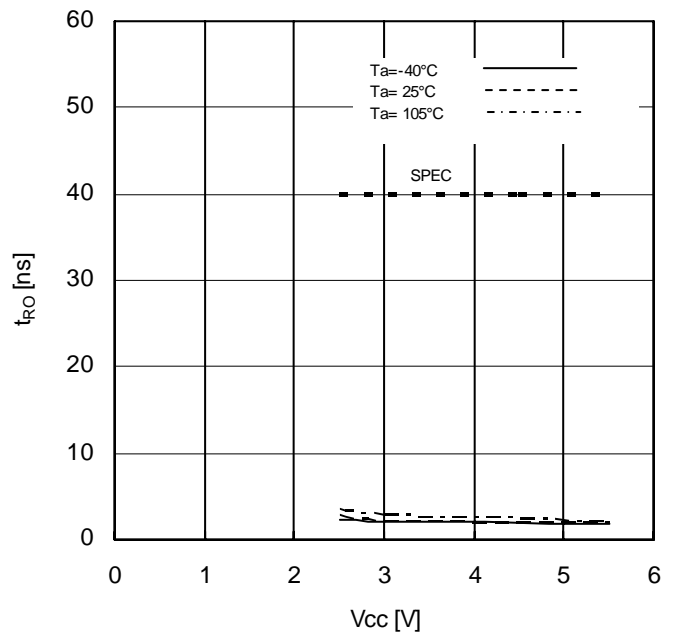
Figure 28. OUTPUT Rise Time vs Supply Voltage
