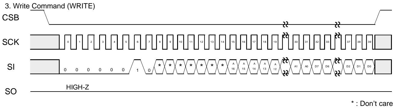
Figure 34. Write command
