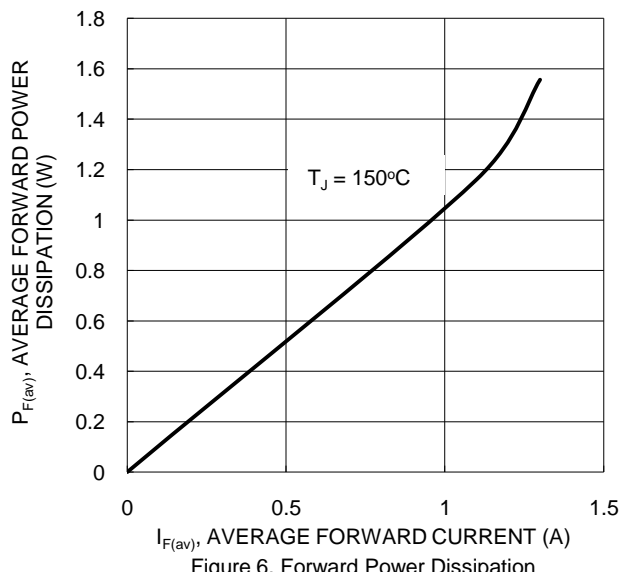
Figure 6. Forward Power Dissipation
