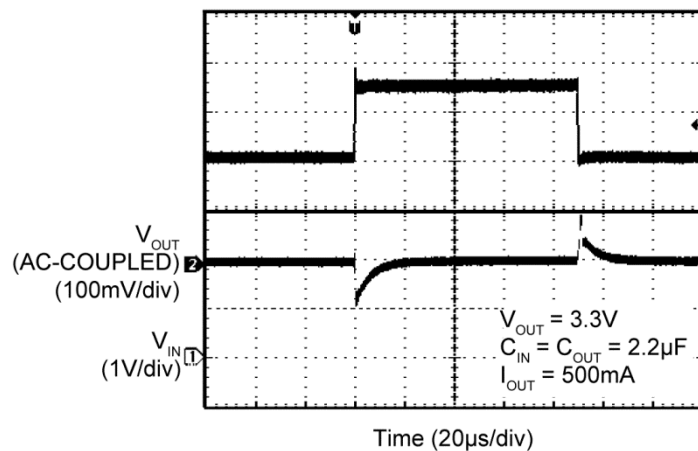
Line Transient
