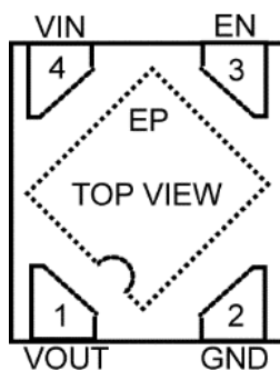
4-Pin 1mm × 1mm Thin DFN (MT) (Top View)
