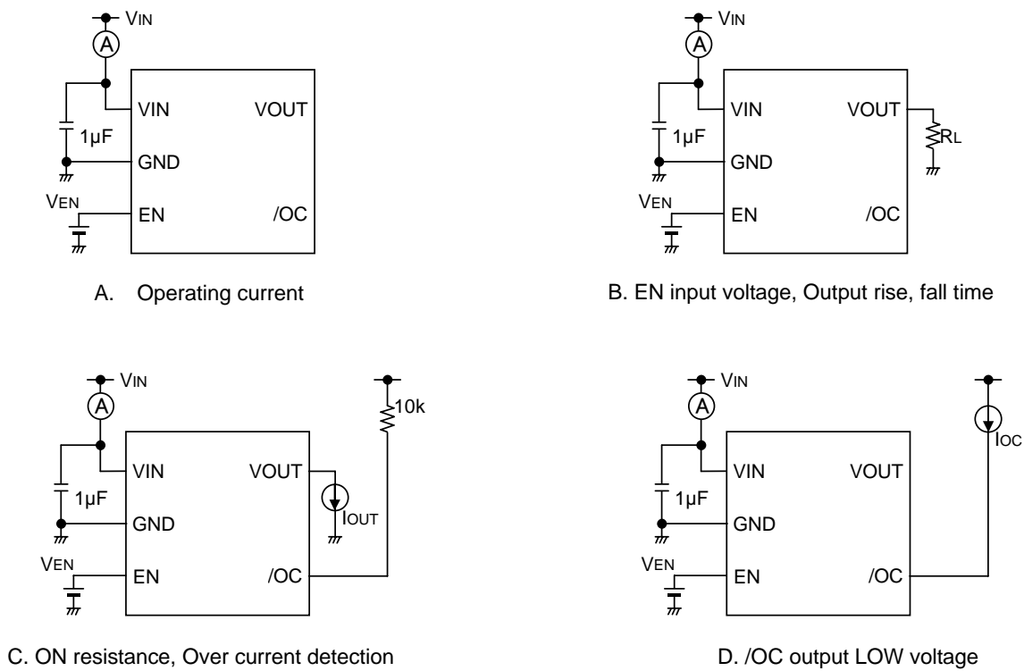
Figure 1. Measurement circuit
