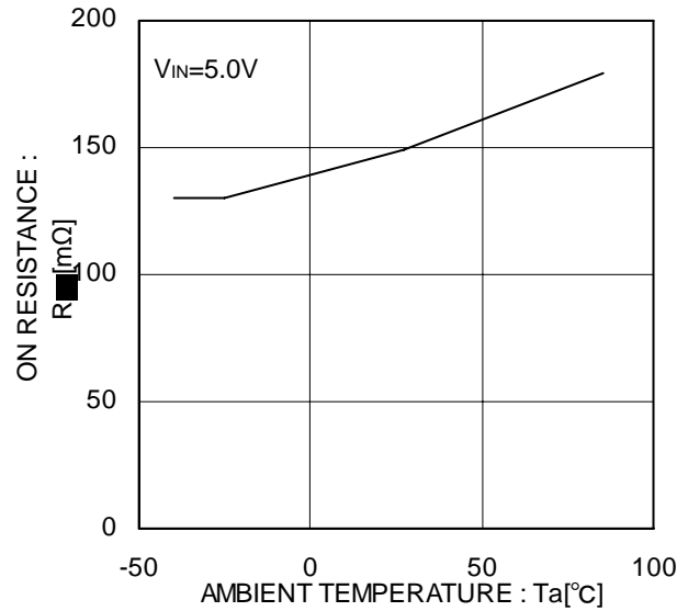
Figure 10. ON resistance
