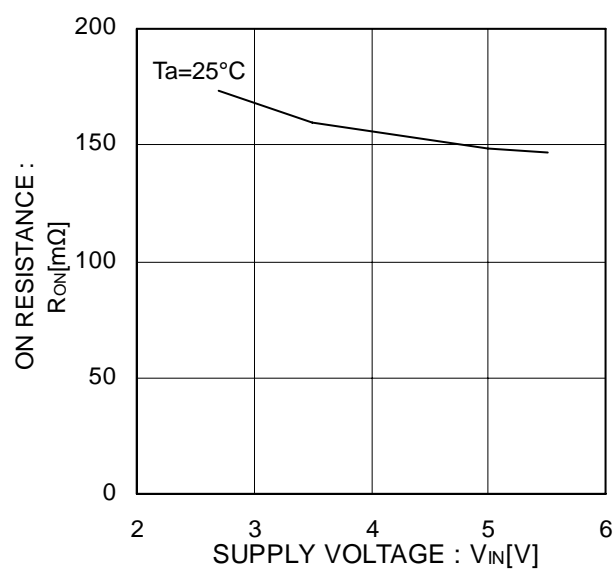
Figure 9. ON resistance
