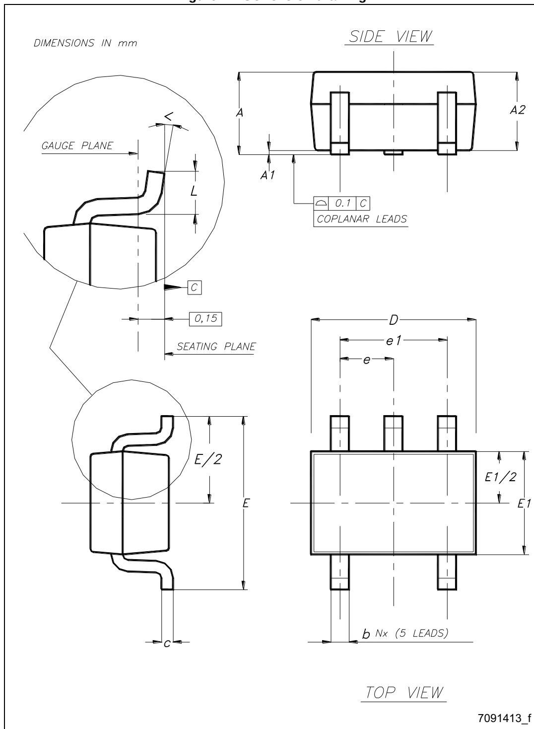
Figure 17. SOT323-5L drawing
