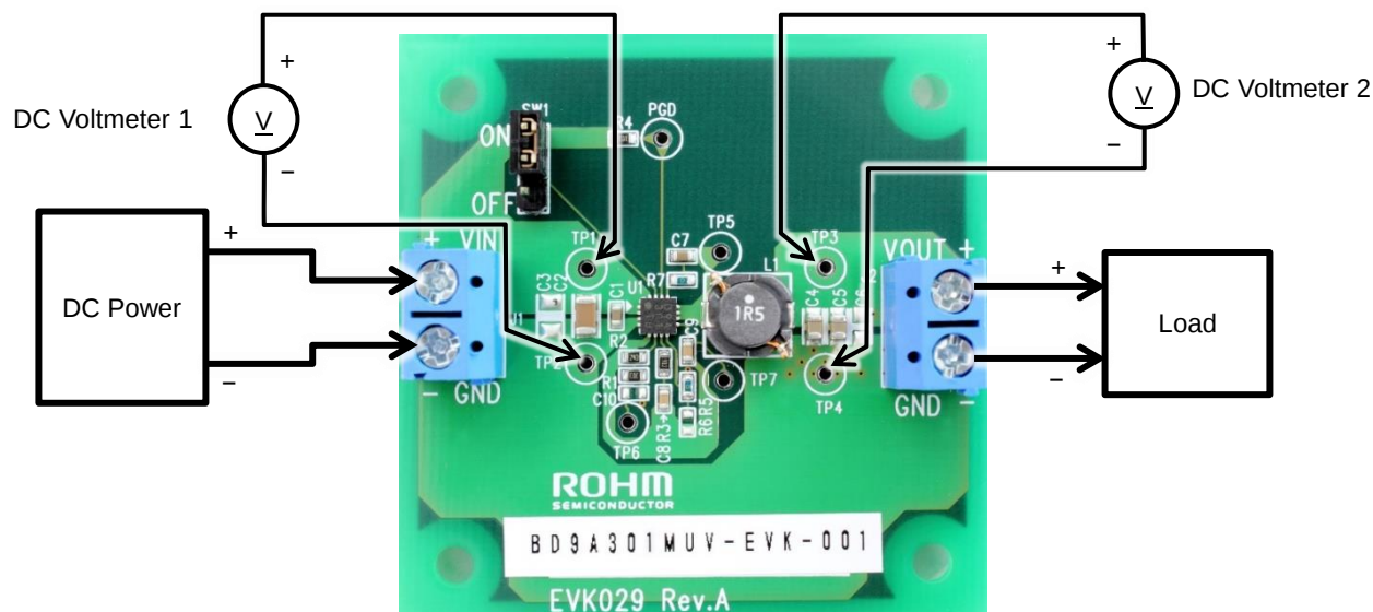
Figure 1. Connection Diagram
