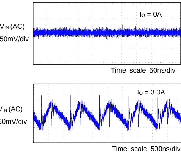
Figure 15. Input Voltage Ripple Wave V_{IN} = 3.3V , V_O = 1.8V
