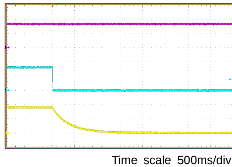
Figure 24. Power-down by EN V_{IN} = 3.3V , V_O = 1.8V , I_O = 0A
