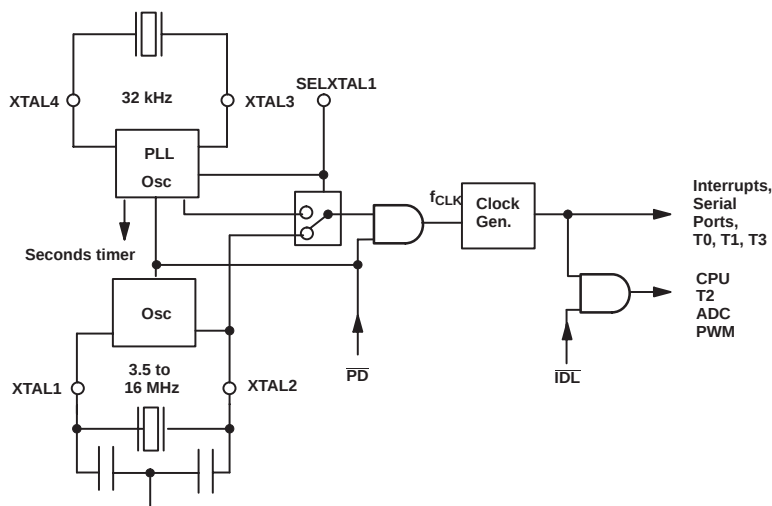
Figure 40. Idle and Power Down Hardware for Clock Generation
