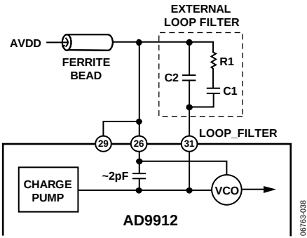
Figure 46. External Loop Filter for SYSCLK PLL
