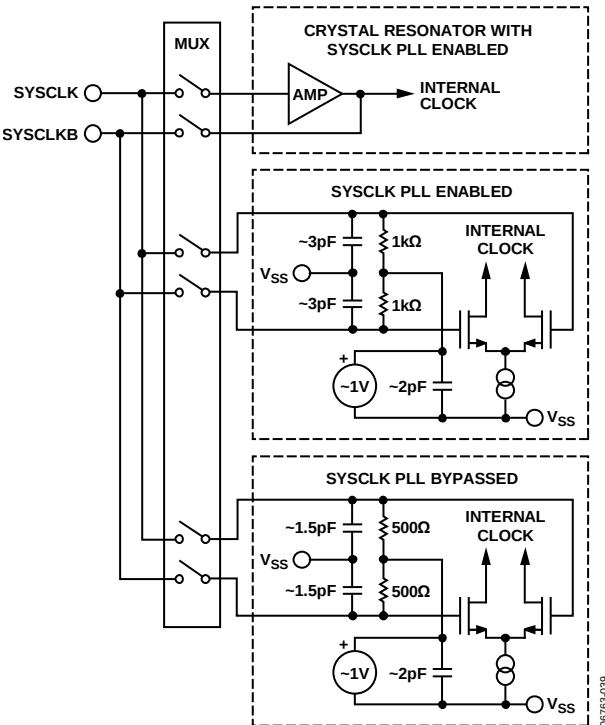
Figure 47. Differential SYSCLK Inputs
