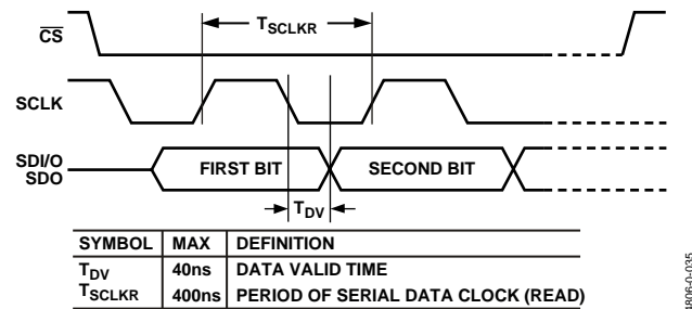
Figure 41. Timing Diagram for Data Read to AD9540
