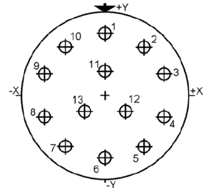
D38999 Series III MIL-STD-1560 Arrangement 11-35 (Mating face - PIN insert shown)
