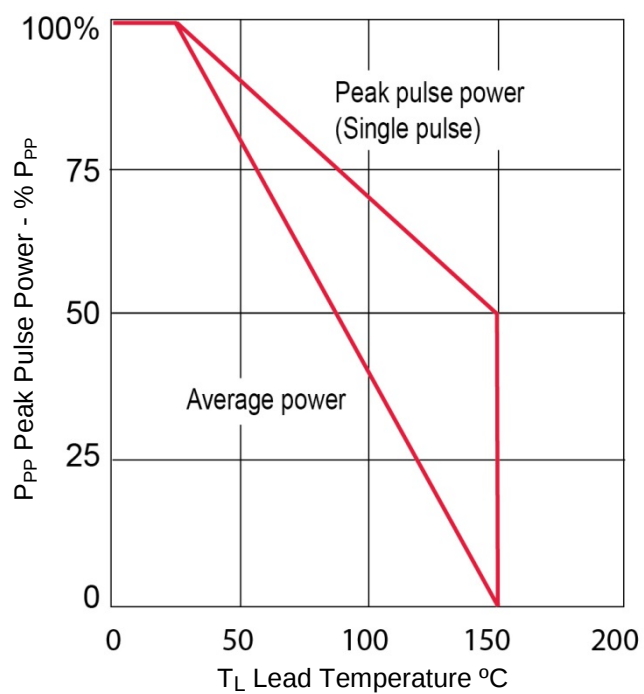
FIGURE 3 Derating Curve
