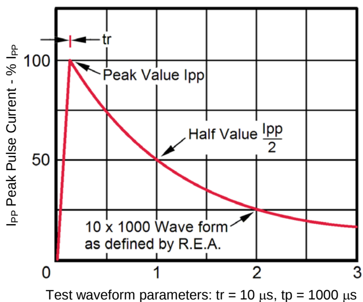
FIGURE 2 Pulse Waveform
