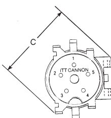
Front-Face View 5 Cavity Housing
