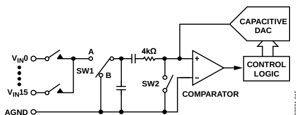
Figure 16. ADC Conversion Phase
