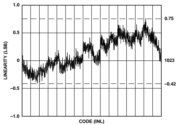
Figure 18. Typical Linearity
