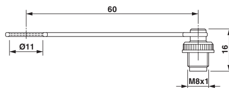
Dimensional drawing
