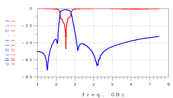
RFBPF1608060K2T
