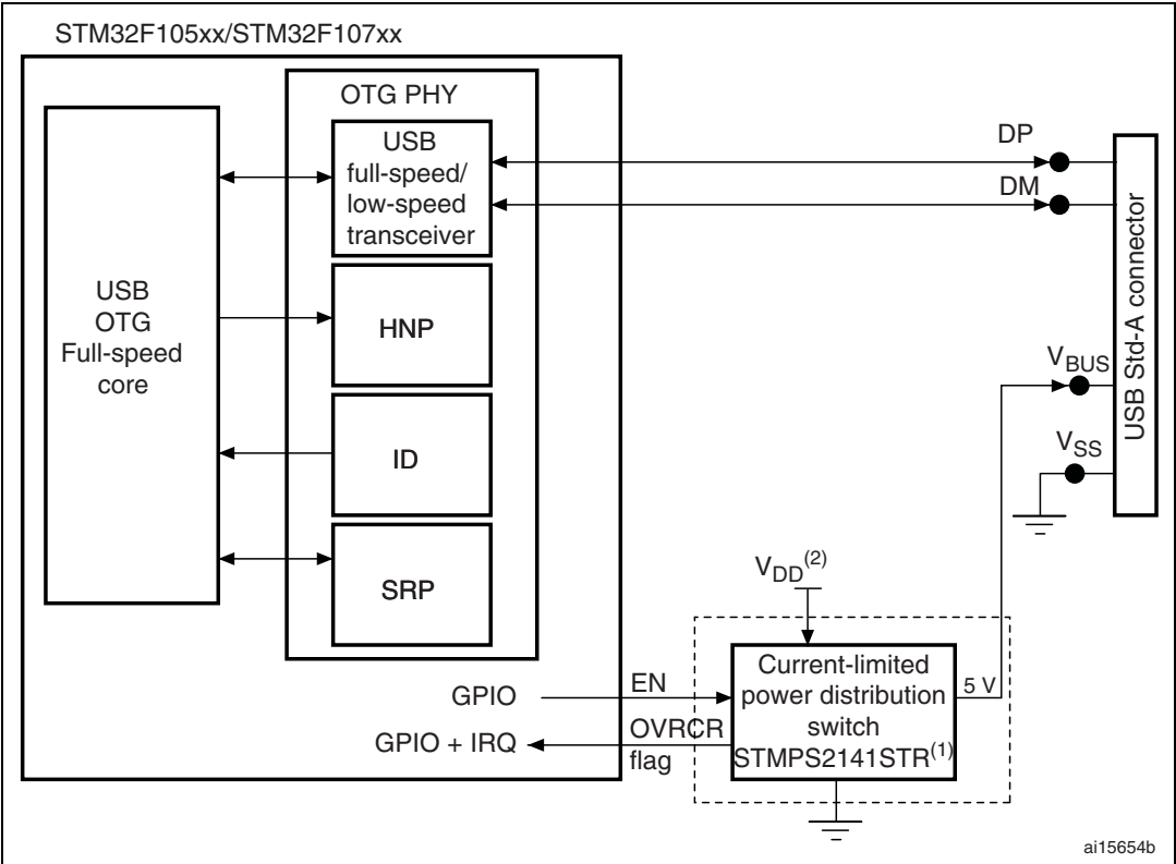
Figure 47. Host connection
