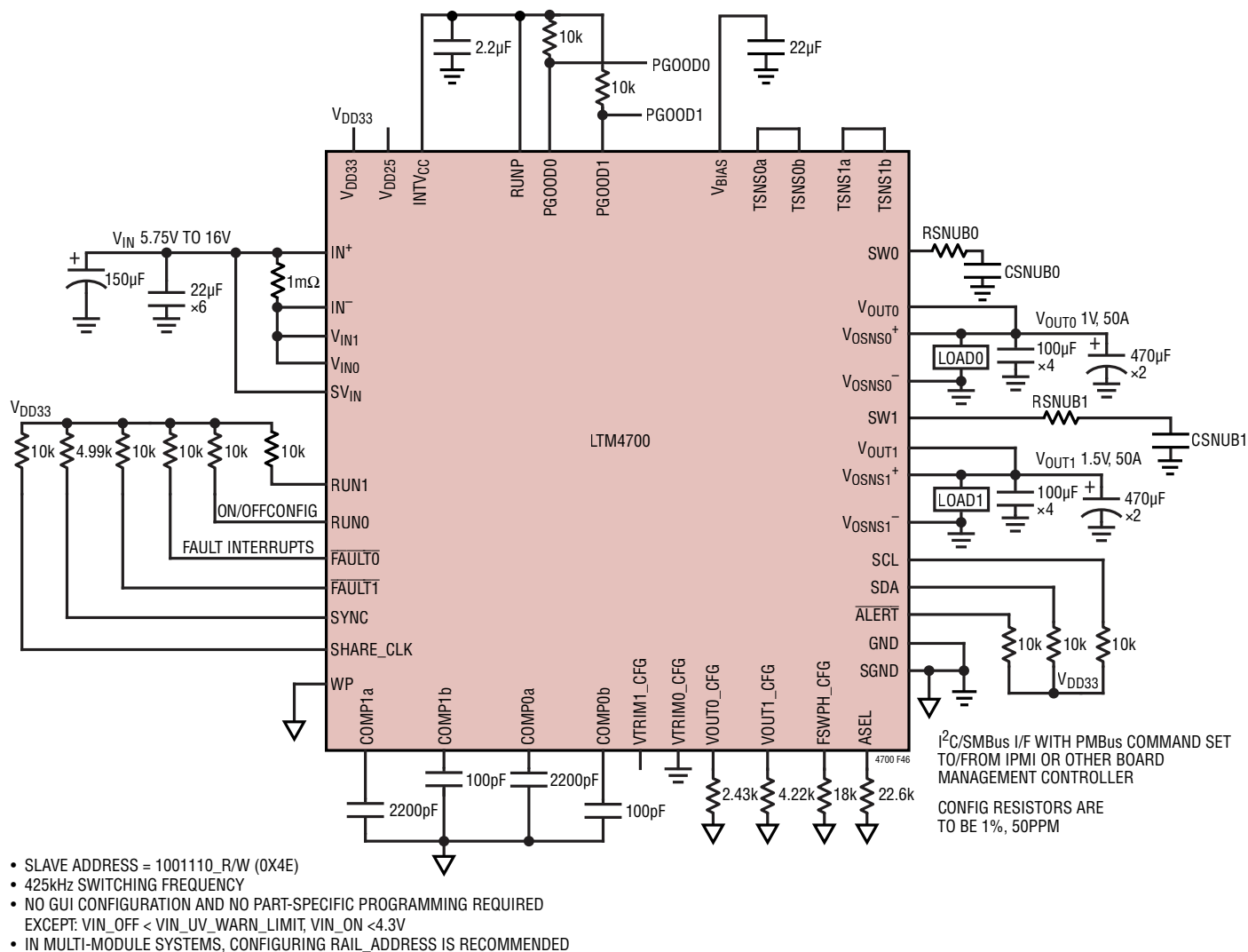
Figure 46. 1.0V and 1.5V Outputs at 50A With Providing I 2 C/SMBus/PMBus Serial Interface
