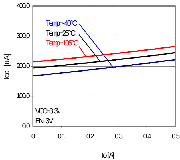
Figure 30. I_O-I_{CC}
