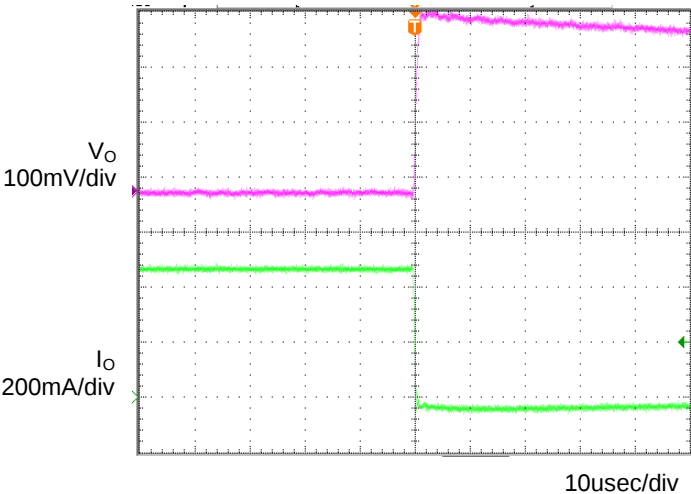
Figure 8. Transient Response (0.5→0A) C_o=1\mu\text{F} , T_a=105^\circ\text{C}
