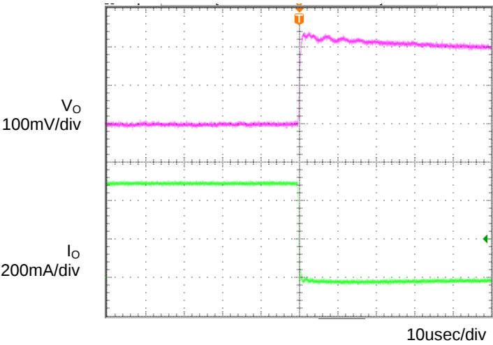
Figure 7. Transient Response (0.5→0A) C_o=1\mu\text{F} , T_a=25^\circ\text{C}
