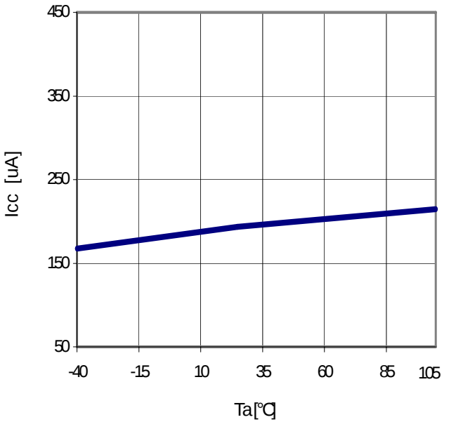
Figure 22. T_a - I_{CC}
