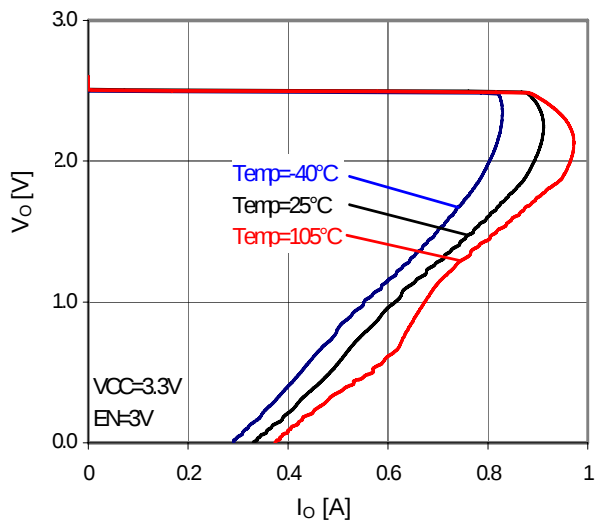
Figure 29. OCP
