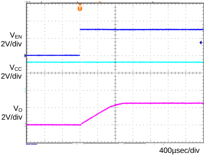
Figure 16. Input sequence 2 C_o=1\mu\text{F} , T_a=25^{\circ}\text{C}
