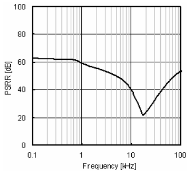
Figure 32. PSRR (Io=0mA)
