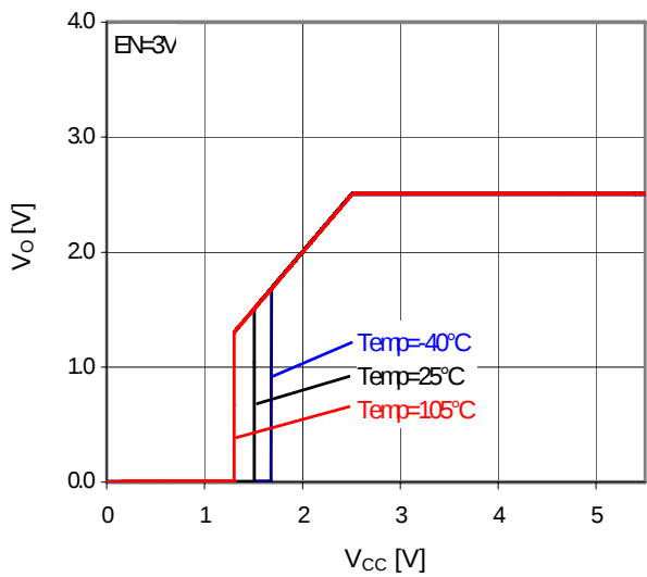
Figure 27. V_{CC}-V_O ( I_O=0mA )
