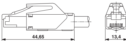
Dimensioned drawing
