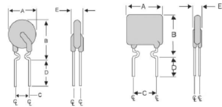
Fig.1 Lead Size: 24AWG Ø0.51 mm Diameter
