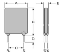
Fig.4 Lead Size: 18AWG Ø1.00 mm Diameter
