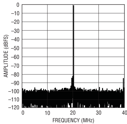
LTC2259-12: 8k Point FFT, f_{IN} = 140\text{MHz} , -1\text{dBFS} , 80Msps
