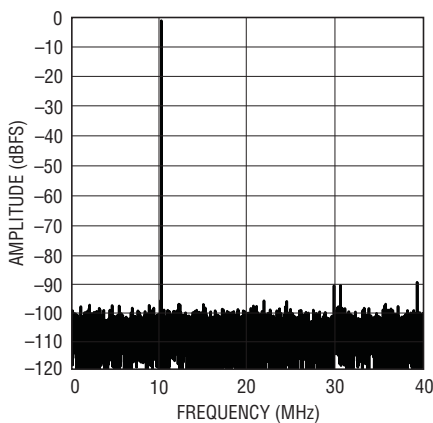
LTC2259-12: 8k Point FFT, f_{IN} = 70\text{MHz} , -1\text{dBFS} , 80Msps
