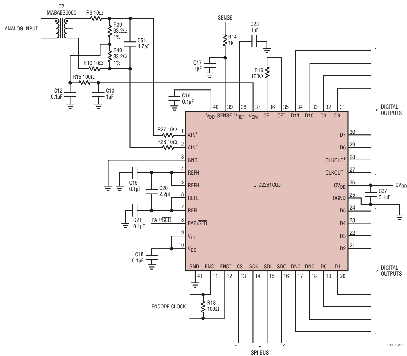
LTC2261 Schematic
