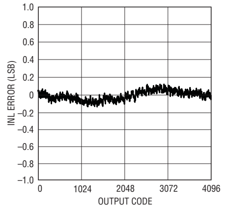
LTC2259-12: Integral Nonlinearity (INL)
