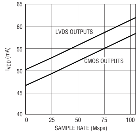
LTC2260-12: I_{VDD} vs Sample Rate, 5\text{MHz Sine Wave Input, -1dB}
