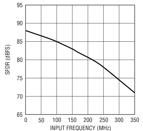
LTC2259-12: SFDR vs Input Frequency, -1\text{dB} , 2V Range, 80Msps
