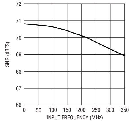
LTC2260-12: SNR vs Input Frequency, -1dB, 2V Range, 105\text{Mpsps}
