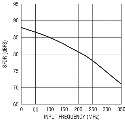
LTC2260-12: SFDR vs Input Frequency, -1dB, 2V Range, 105\text{Mpsps}
