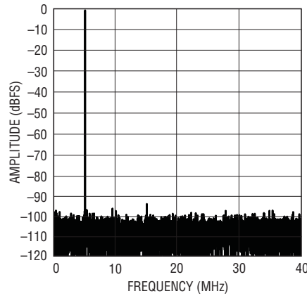
LTC2259-12: 8k Point FFT, f_{IN} = 5\text{MHz} , -1\text{dBFS} , 80Msps
