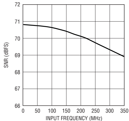
LTC2259-12: SNR vs Input Frequency, -1\text{dB} , 2V Range, 80Msps
