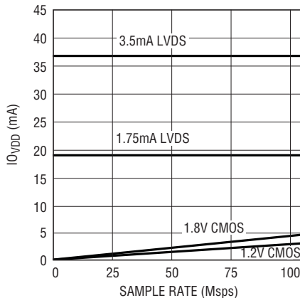
LTC2260-12: I_{O_{VDD}} vs Sample Rate, 5MHz Sine Wave Input, -1\text{dB}, 5\text{pF on Each Data Output}
