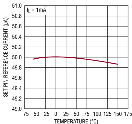
SET Pin Reference Current
