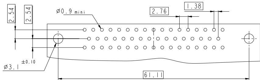
LAYOUT DIMENSIONS
