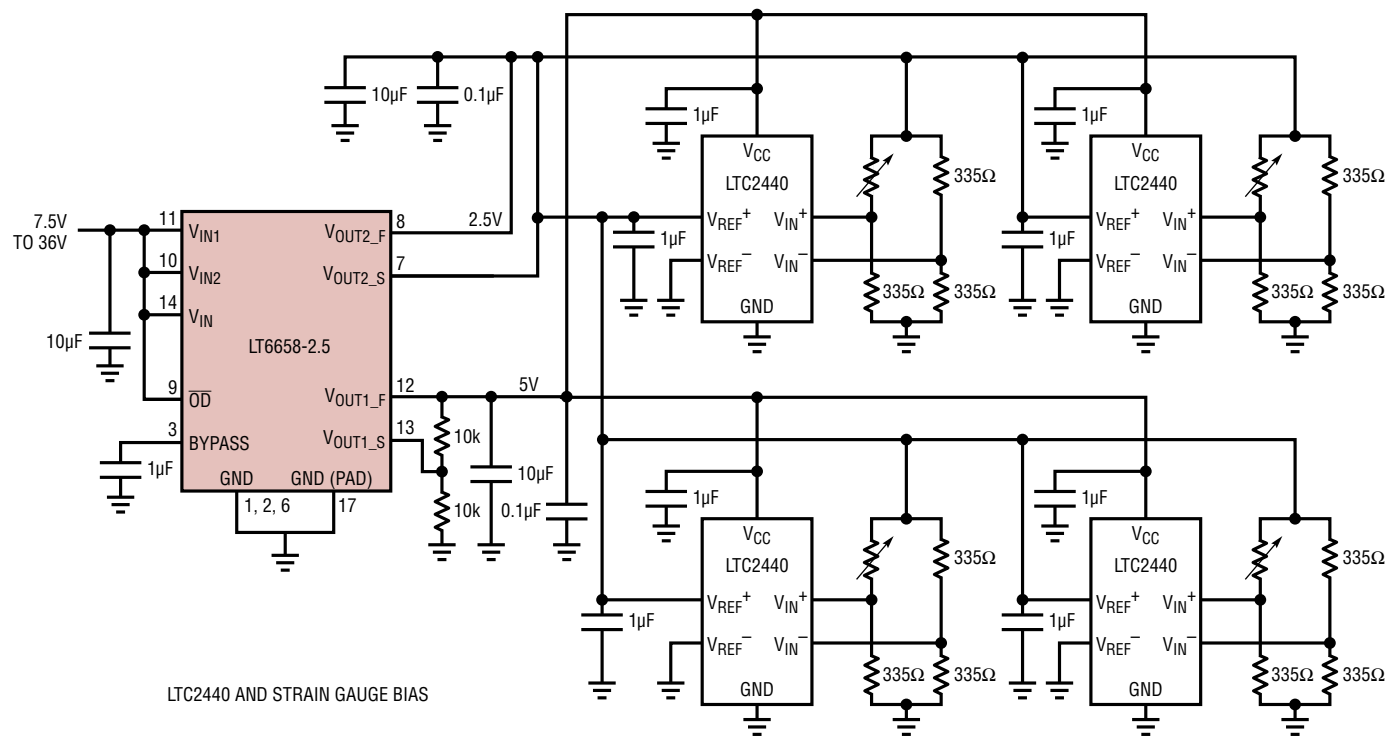
LT6658 Biasing Multiple Strain Gauges
